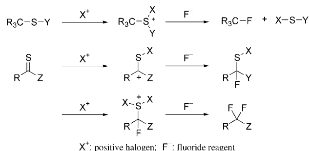
Scheme 1. Oxidative desulfurization-fluorination of organosulfur compounds.
