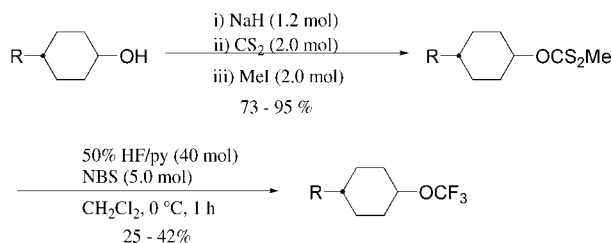
Scheme 9. Synthesis of trifluoromethoxycyclohexane-type liquid crystals.
