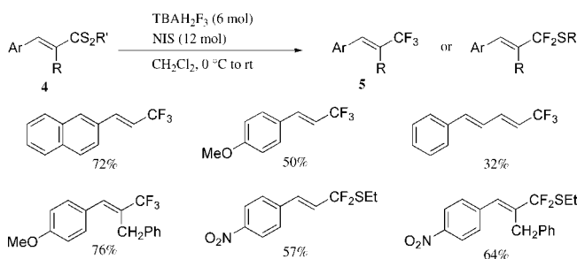
Figure 4. Trifluorination or difluorination of \alpha,\beta -unsaturated dithiocarboxylates.
