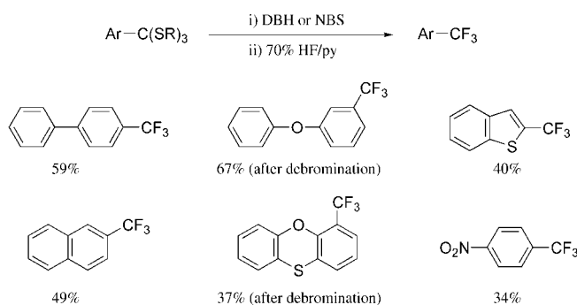
Figure 5. Oxidative desulfurization-fluorination of orthothioesters.
