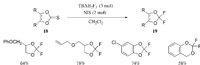
Figure 10. Synthesis of carbonyl fluoride acetals by oxidative desulfurization-fluorination.
