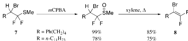
Scheme 6. Synthesis of 2-bromo-1,1-difluoro-1-alkenes.
