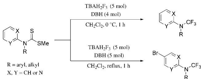
Scheme 8. Synthesis of trifluoromethylamines.
