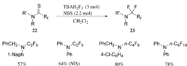
Figure 11. Preparation of perfluoroalkylamines 23 .
