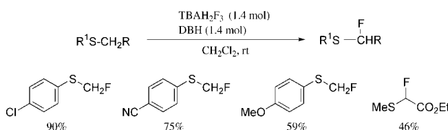
Figure 1. Fluoro-Pummerer rearrangement of sulfides.
