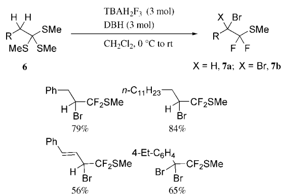
Figure 6. Brominative fluorination of orthothioesters.
