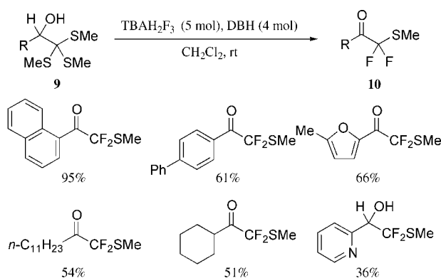
Figure 7. Oxidative desulfurization-fluorination of 2,2,2-tris(methylthio)ethanols.
