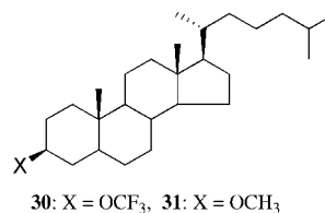
Figure 13. Chiral dopants for TN- and TFT-TN-LC displays.
