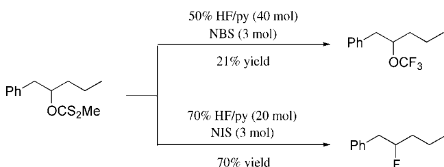
Scheme 7. Synthesis of secondary alkyl fluorides or trifluoromethyl ethers from dithiocarbonates.
