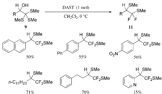
Figure 8. Fluorination of 2,2,2-tris(methylthio)ethanols with DAST.
