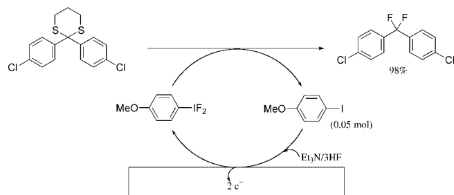
Scheme 3. Electrochemical fluorination of dithioacetals.
