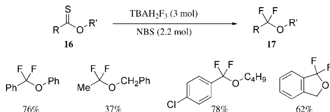
Figure 9. Synthesis of α,α-difluoro ethers by oxidative desulfurization-fluorination.
