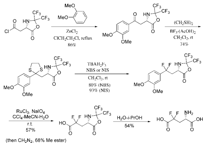
Scheme 2. Synthesis of difluoroglutamic acid from aspartic acid.
