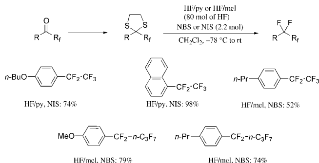
Figure 3. Synthesis of perfluoroalkyl-substituted aromatic compounds.
