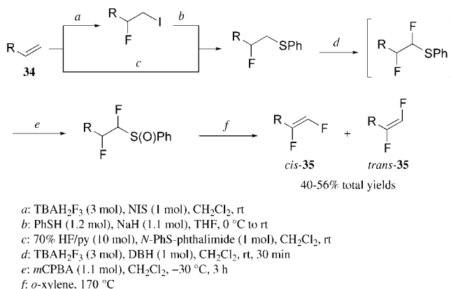
Scheme 10. Synthesis of vic -difluoro-olefins from terminal olefins.
